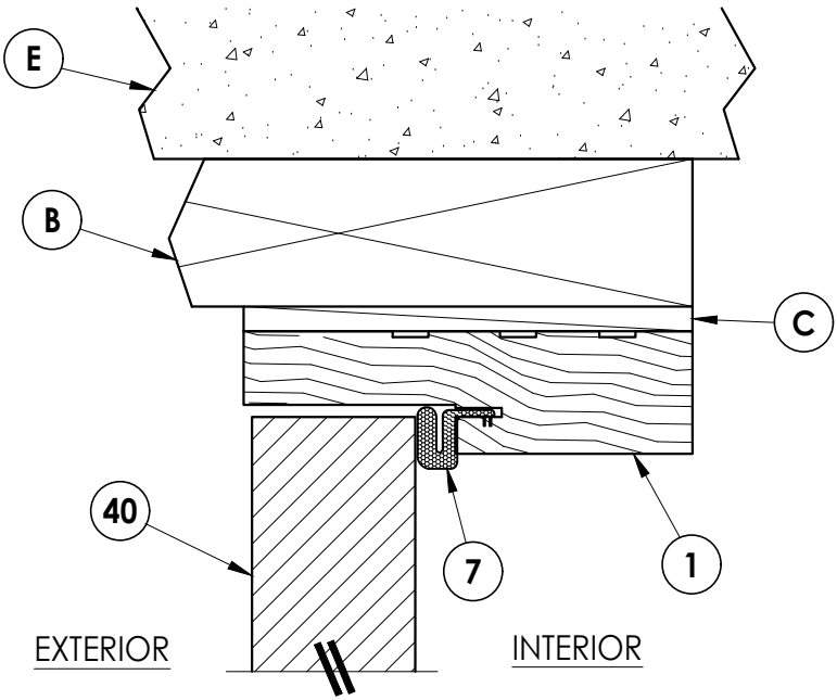
1 5 VERTICAL CROSS SECTION Outswing shown (Inswing similar)
